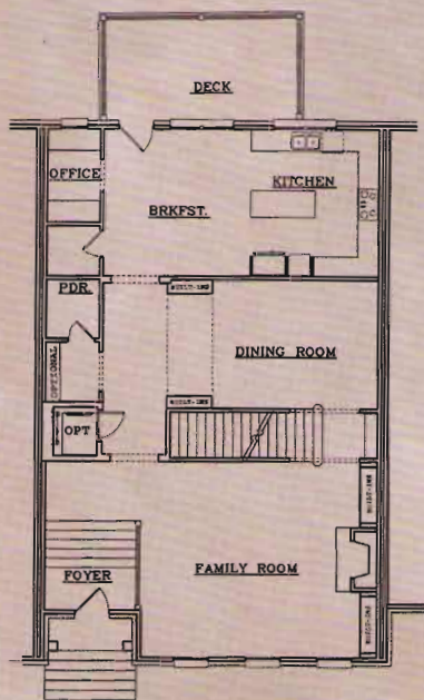
MAIN LEVEL PLAN THE DEVONSHIRE
