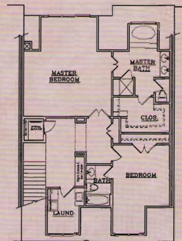
UPPER LEVEL PLAN THE BENNETT Variations on upper level plans available, see agent for details.
